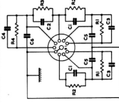
SINGLE LETTER ADAPTOR
